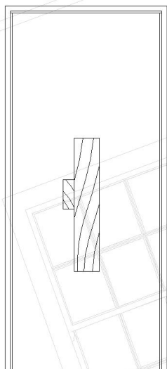
Door Lining 145 x 28 with loose stops (Deeper linings available)
